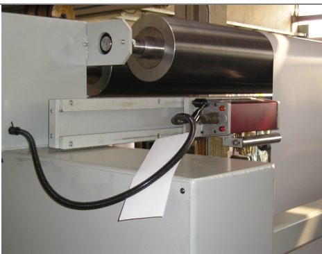
Model 1032 Classic® Splice Detector™ MWU Sheeter
